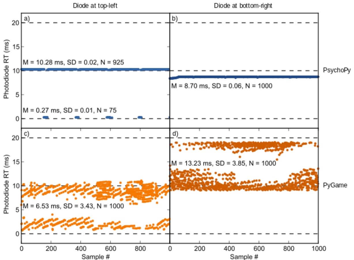
Figure 2. Results of a benchmark experiment for temporal precision and accuracy of display presentation times obtained with PyGaze, using either PsychoPy or PyGame.
