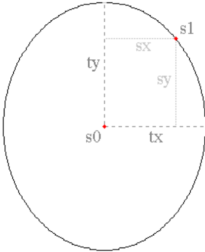
Figure 1. Two gaze position samples s_0 and s_1 with their corresponding horizontal and vertical inter-sample distances s_x and s_y ; t_x and t_y represent the horizontal and vertical thresholds for RMS noise
